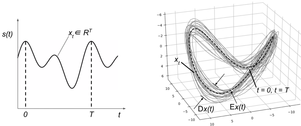
Рис. 1. Time series and phase trajectory
