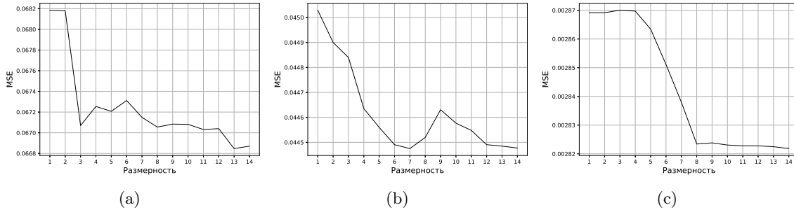
Рис. 3. Error value depending on the dimensionality of the trajectory space: (a) accelerometer, walking, (b) accelerometer, running, (c) energy consumption
